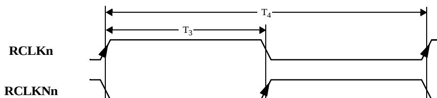
Figure 19: RCLKn and RCLKNn Timing Waveforms with DUAL = 1
