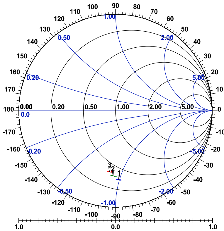
Figure 9.3: TX_A PL35
