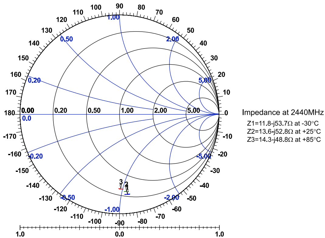
Figure 9.9: RX_A Balanced
