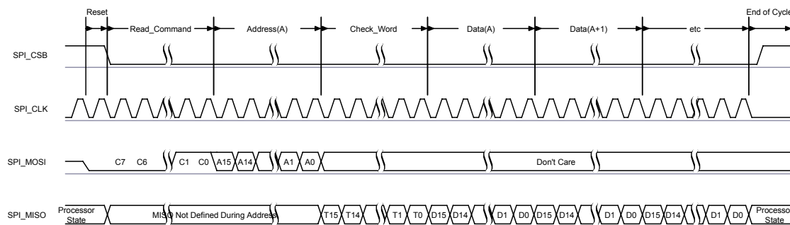
Figure 9.26: Read Operation
