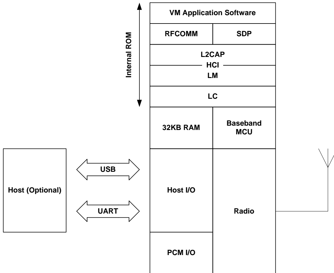
Figure 8.3: Virtual Machine
