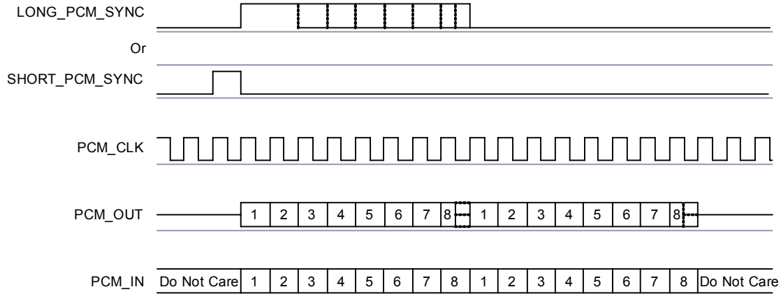
Figure 9.31: Multi Slot Operation with Two Slots and 8-bit Companded Samples
