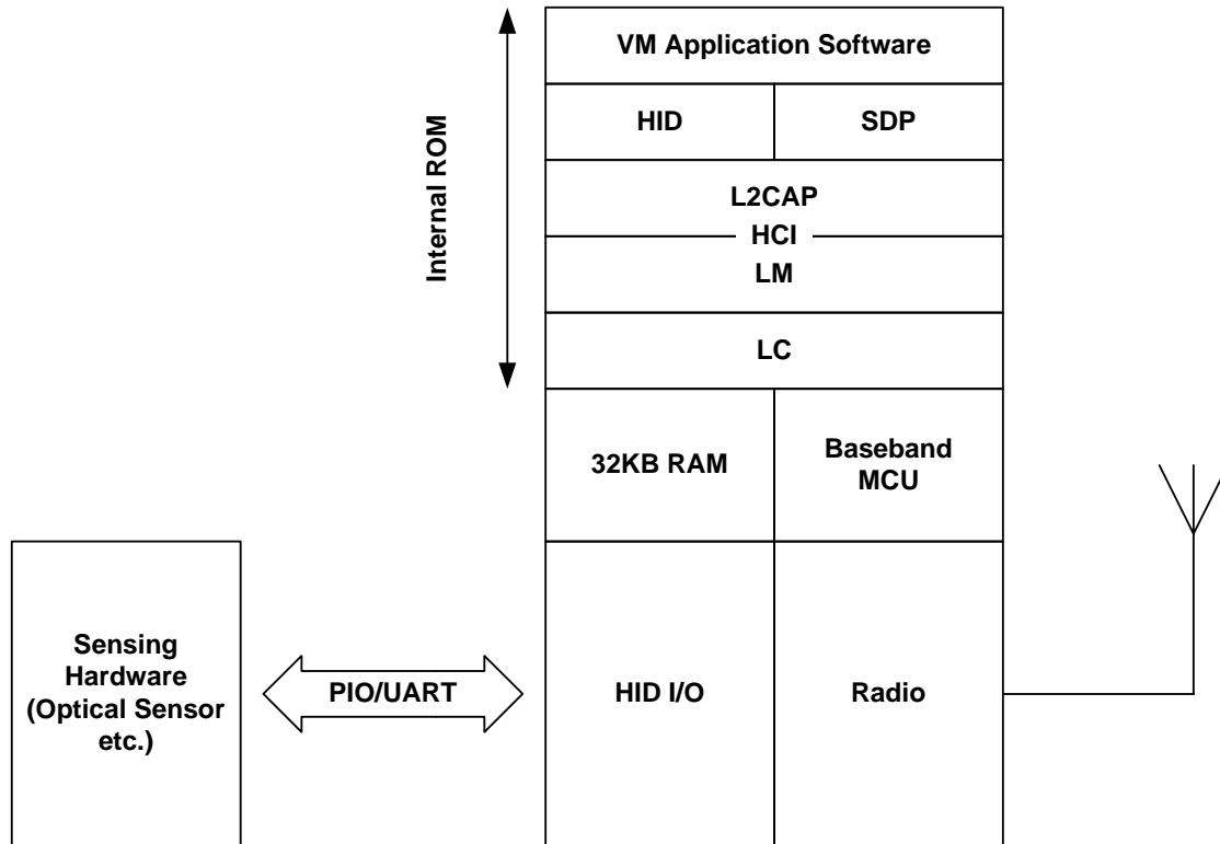
Figure 8.4: HID Stack
