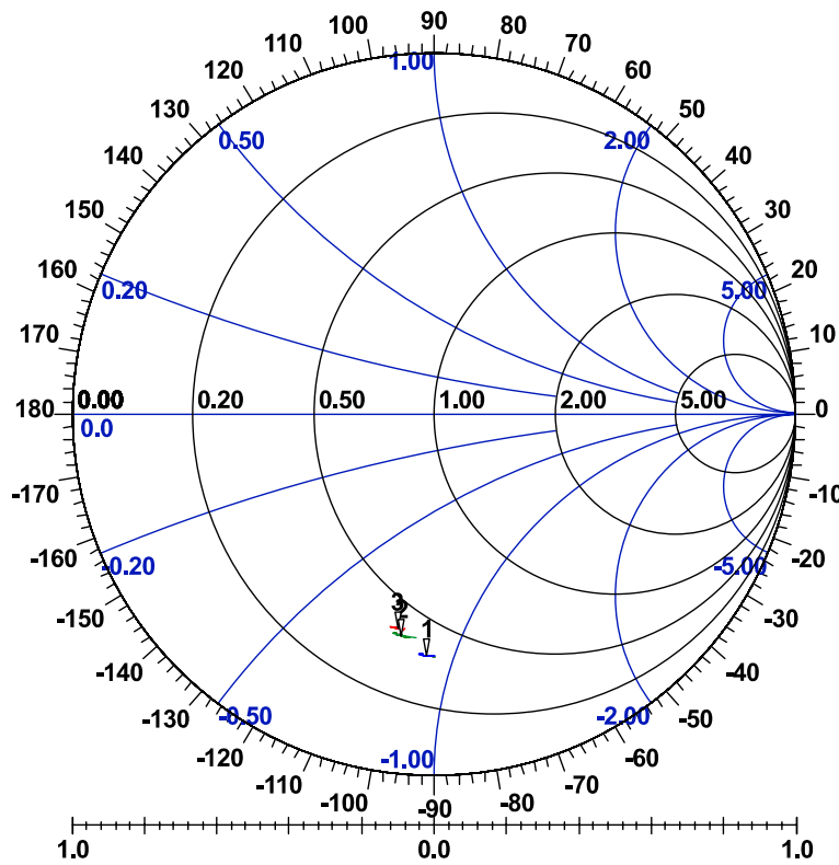
Figure 9.5: TX_A PL63
