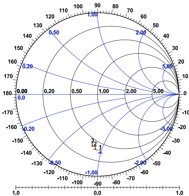
Figure 9.4: TX_A PL50
