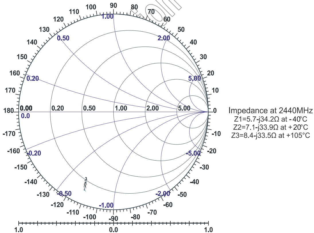
Figure 8.10: RX_B Balanced Receive Input Impedance
