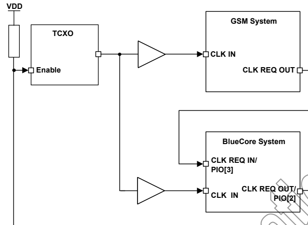
Figure 8.37: Example TXCO Enable OR Function
