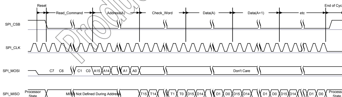
Figure 8.25: Read Operation
