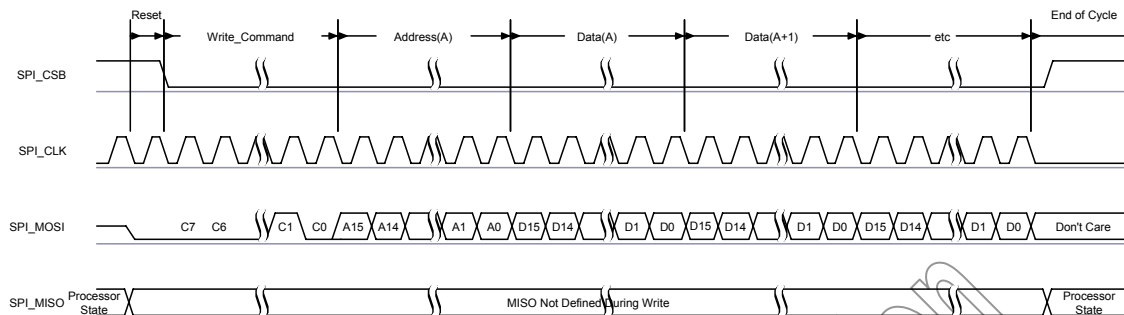
Figure 8.24: Write Operation
