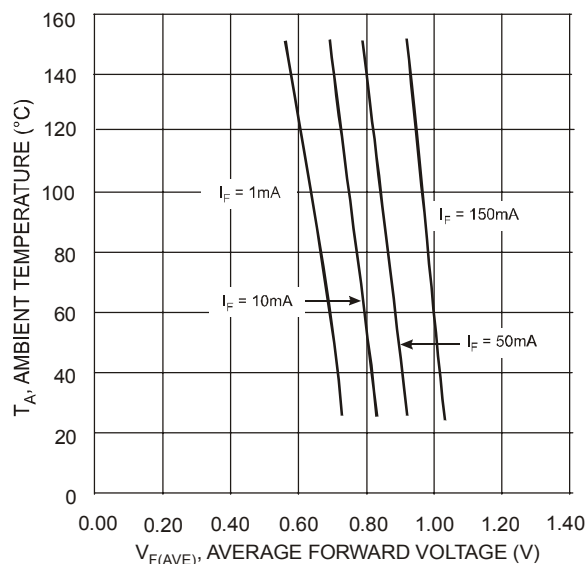
Fig. 4 Typical Forward Voltage vs Ambient Temperature
