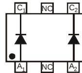
Device Schematic
