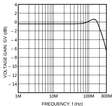
Fig. 4 Frequency characteristics
