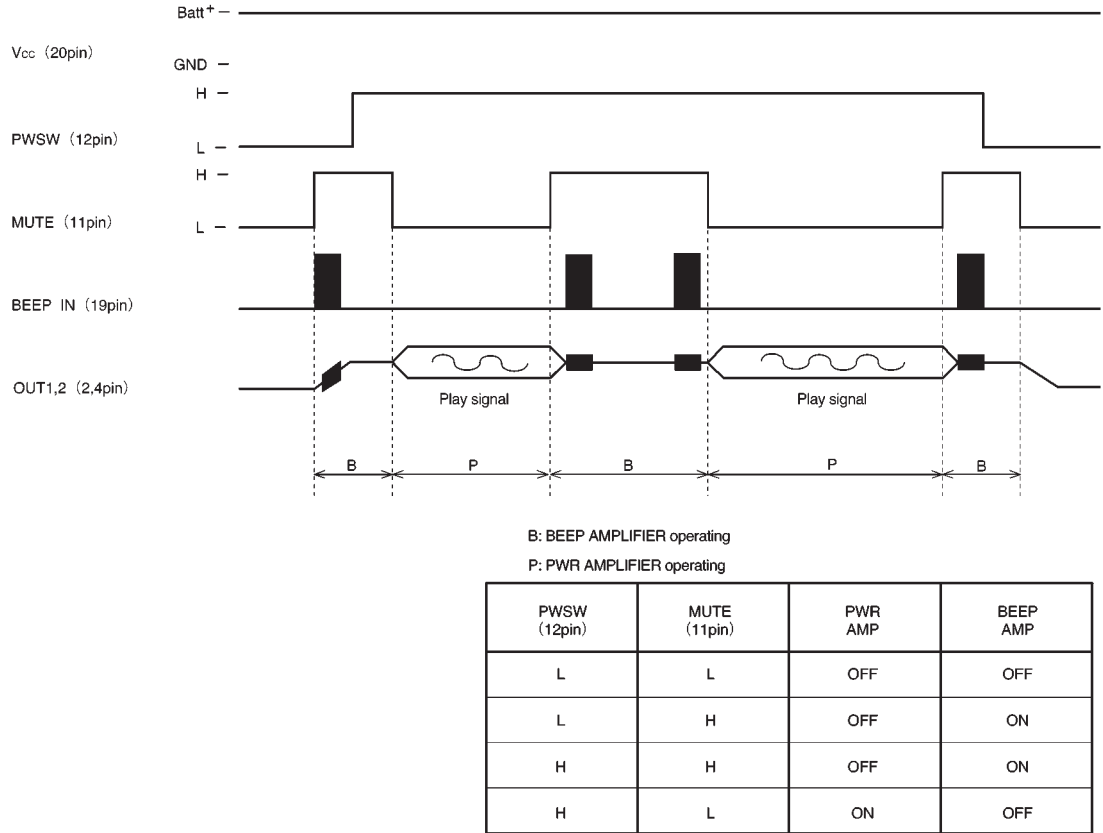
Fig.3 Time chart
