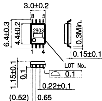
BA2903FV (SSOP-B8) (Unit:[mm])
