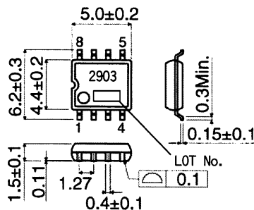
BA2903F (SOP8) (Unit:[mm])
