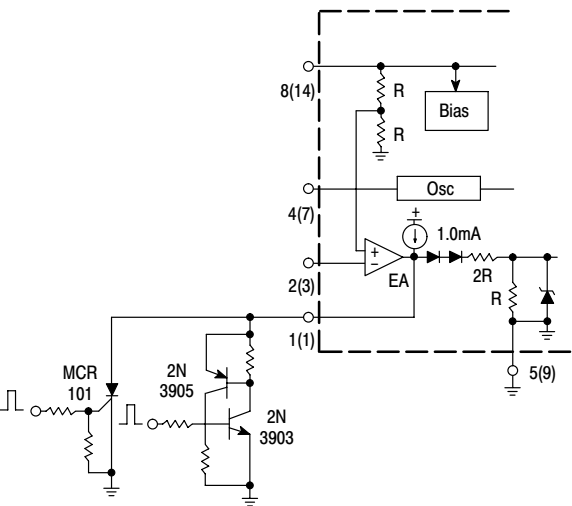
Figure 25. Bipolar Transistor Drive
