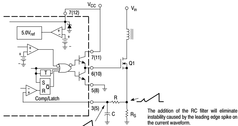
Figure 23. Current Waveform Spike Suppression
