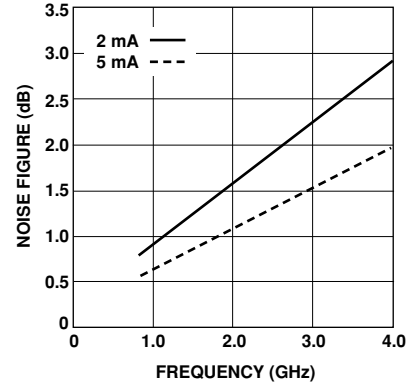
Figure 3. AT-41532 Typical Noise Figure vs. Frequency and Current at 5 V.
