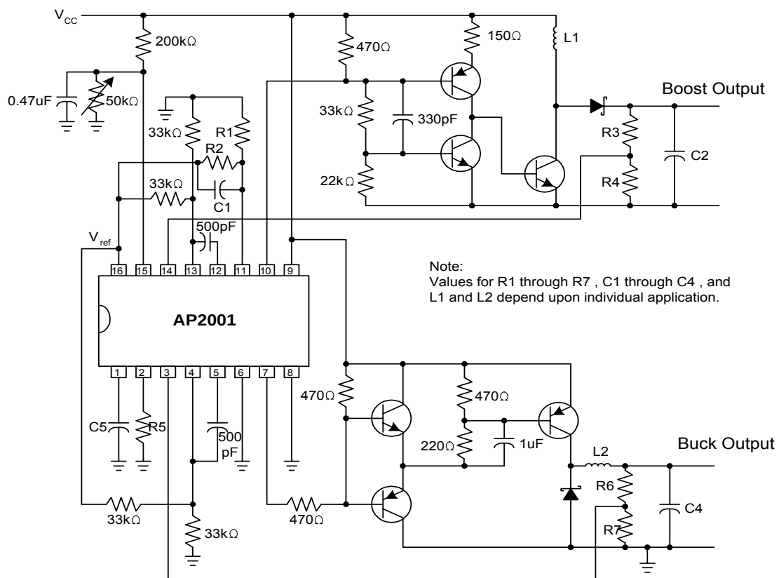
Dual output DC/DC converter
