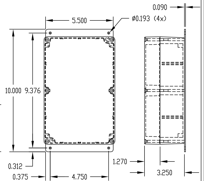
SECTION "D-D"
