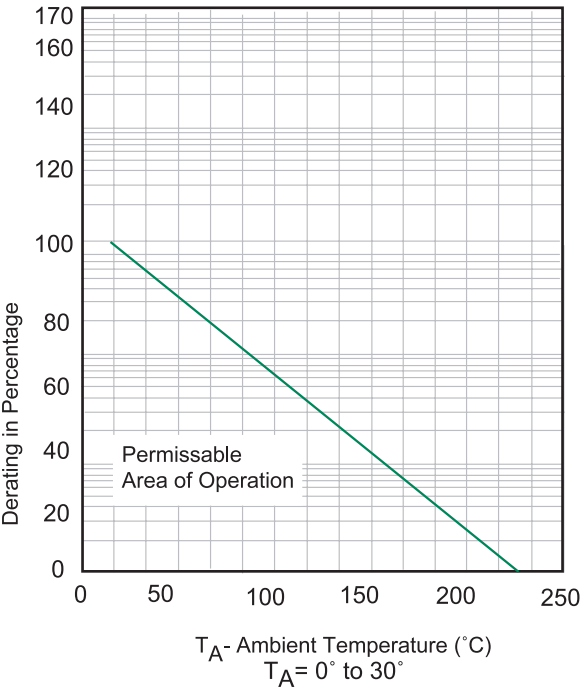
Figure 1. Peak Power Derating Peak Pulse Power in Percent of 25% Rating
