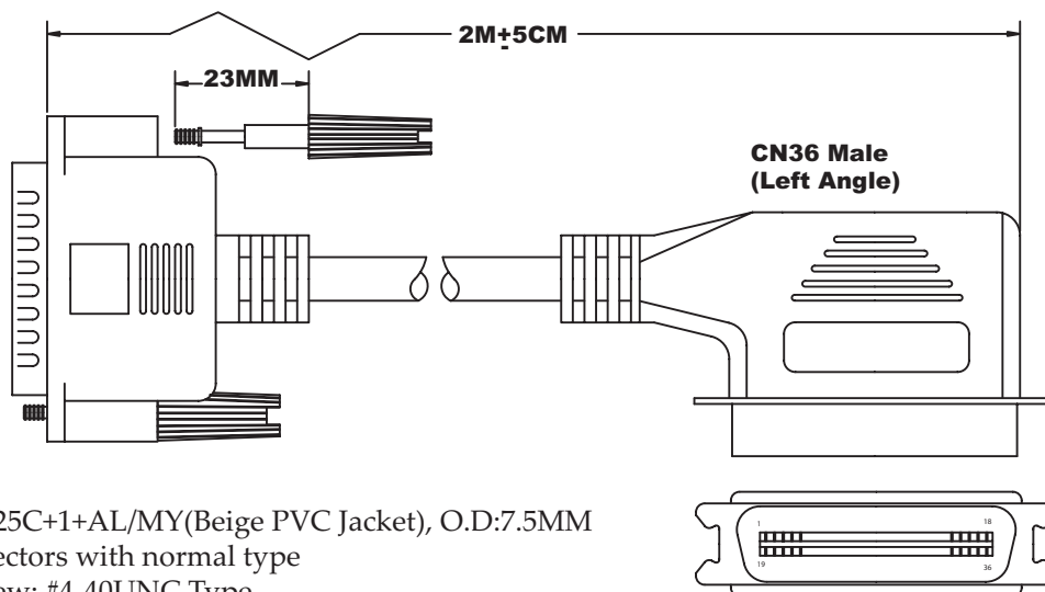
DB25 Male
