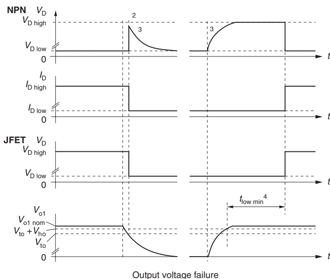
Fig. 33 Relationship between V_i , V_{o1} , V_D , V_{o1}/V_o\text{ nom} versus time
