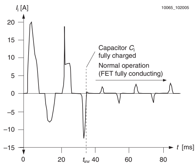
Fig. 26 Inrush current with option E (LK models, V_i = 230 \text{ VAC} , f_i = 50 \text{ Hz} , P_O = P_{O \text{ nom}} )
