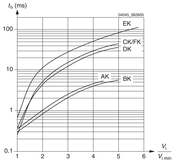
Fig. 6a Typical hold-up time t_h versus relative input voltage V_i/V_{i \min} . The DC-DC converters require an external series diode in the input path if other loads are connected to the same input supply lines.
