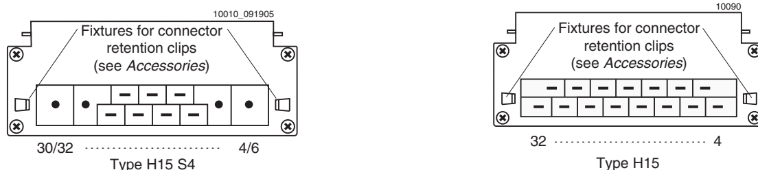
Fig. 21 View of converter's male connectors
