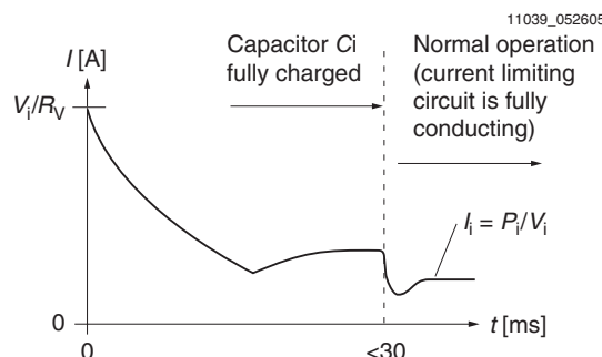
Fig. 25 Inrush current with option E (DC-DC converters)
