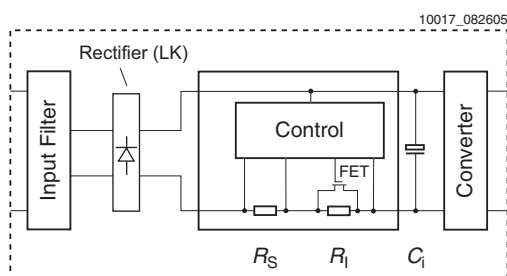
Fig. 24 Option E block diagram
