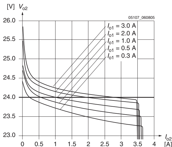
Fig. 12 AK - LK2660: \Delta V_{O2} (typ.) vs. I_{O2} with different I_{O1}
