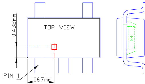
Sensor Location
