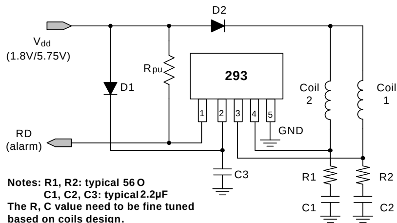
1.8V/5.75V DC Brush-Less Fan with RD Output Function
