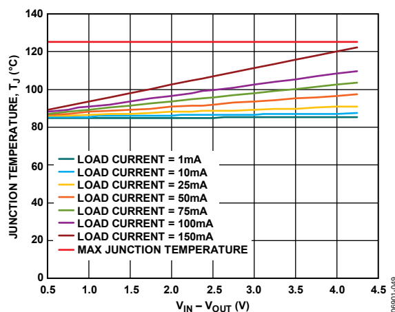
Figure 47. WLCSP, 100 mm² of PCB Copper, T A = 85°C
