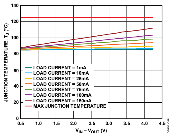
Figure 46. TSOT, 100 mm² of PCB Copper, T A = 85°C
