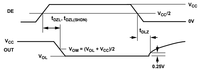
Figure 11. Driver Enable and Disable Times ( t_{DZL} , t_{DZL(SHDN)} , t_{DZL} )
