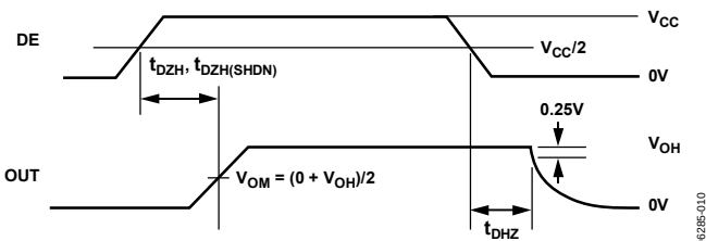
Figure 10. Driver Enable and Disable Times ( t_{DZH} , t_{DZH(SHDN)} , t_{DZH} )
