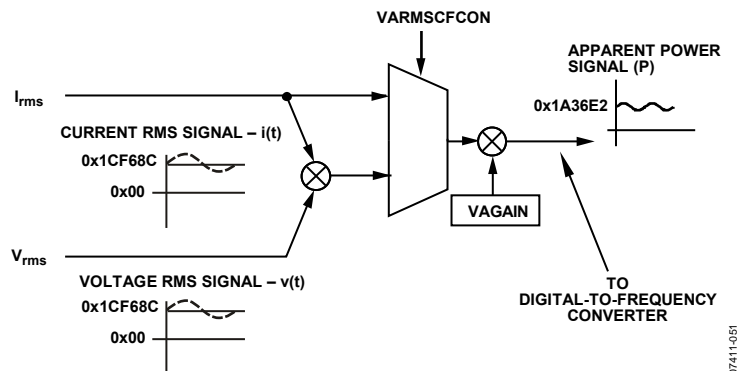
Figure 71. Apparent Power Signal Processing
