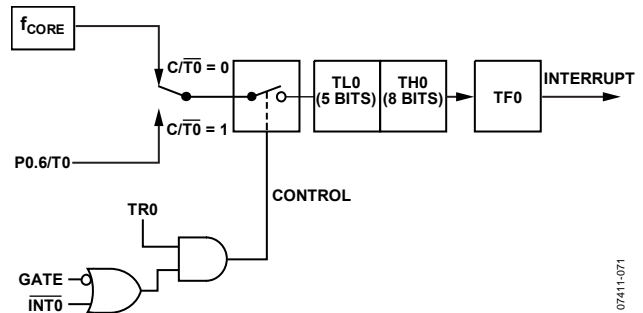
Figure 92. Timer/Counter 0, Mode 0
