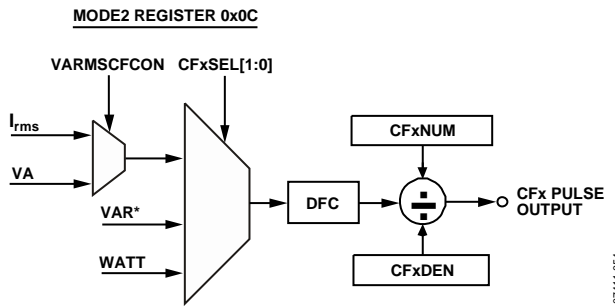
Figure 74. Energy-to-Frequency Conversion
