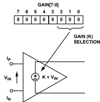
Figure 39. PGA in Current Channel
