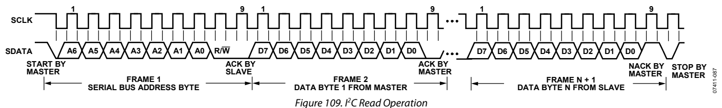
Figure 109. I 2 C Read Operation
