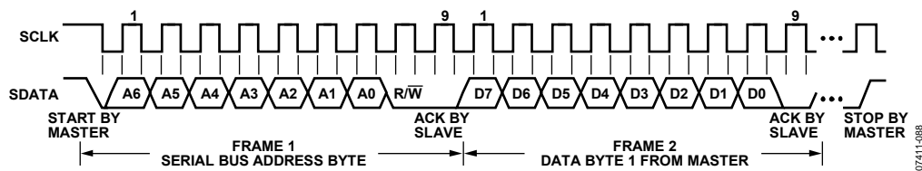
Figure 110. I 2 C Write Operation
