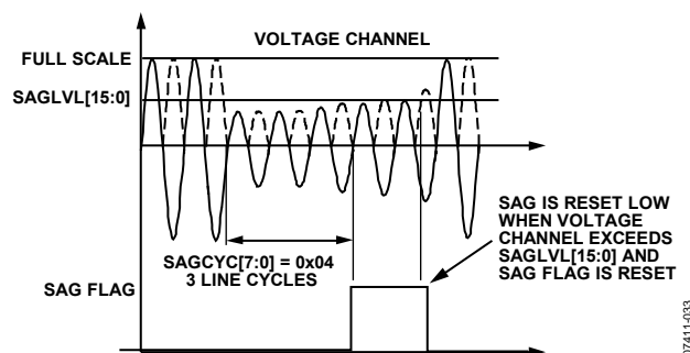
Figure 53. SAG Detection
