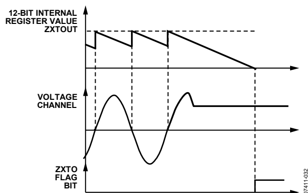
Figure 52. Zero-Crossing Timeout Detection
