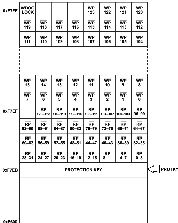
Figure 91. Flash Protection in Page 124
