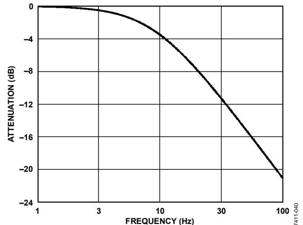
Figure 60. Frequency Response of LPF2
