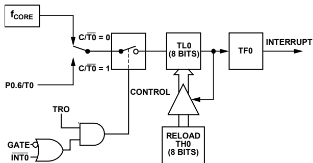
Figure 94. Timer/Counter 0, Mode 2
