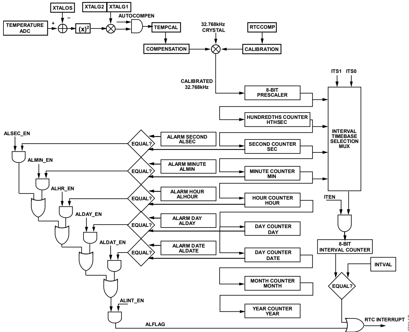
Figure 98. RTC Implementation
