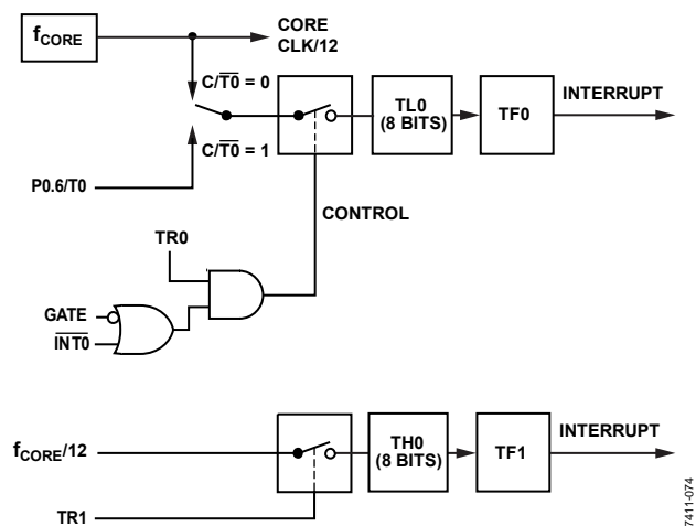
Figure 95. Timer/Counter 0, Mode 3
