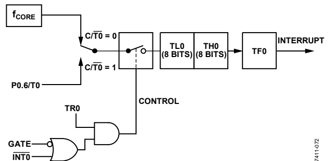
Figure 93. Timer/Counter 0, Mode 1
