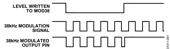
Figure 113. 38 kHz Modulation
