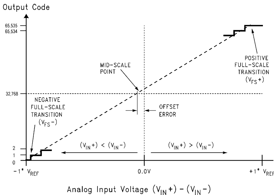
Transfer Characteristic (Offset Binary Format)
