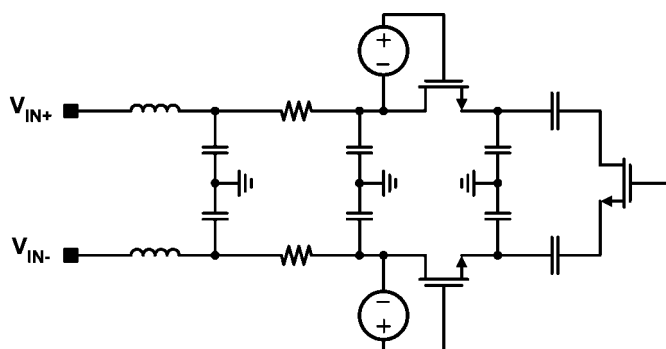
FIGURE 4. Input Equivalent Circuit
