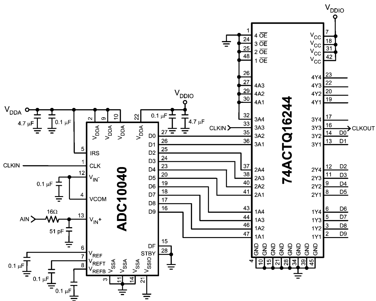
FIGURE 7. A Simple Application Using a Single Ended Signal Source
