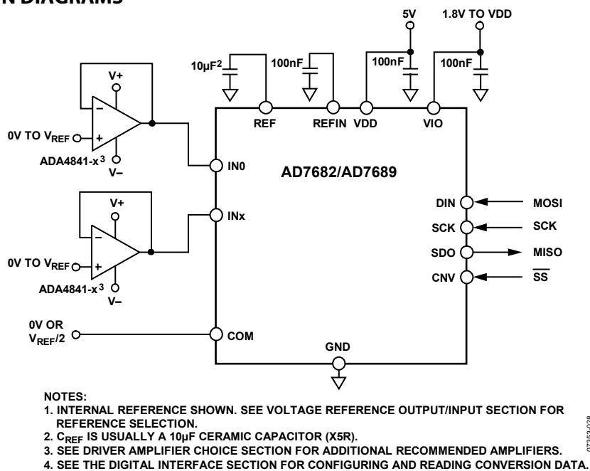
Figure 26. Typical Application Diagram with Multiple Supplies
