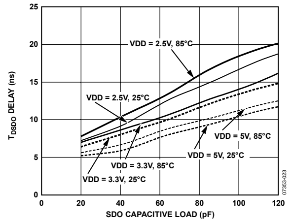
Figure 23. t_{DSO} Delay vs. SDO Capacitance Load and Supply
