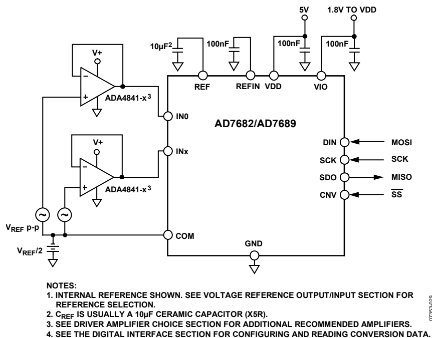
Figure 27. Typical Application Diagram Using Bipolar Input
