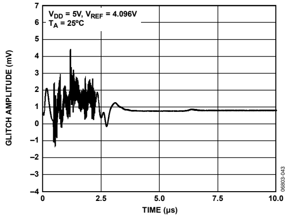
Figure 28. Analog Crosstalk
