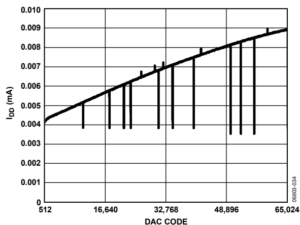
Figure 19. Supply Current vs. Code
