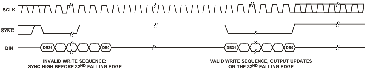
Figure 46. SYNC Interrupt Facility
