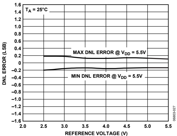
Figure 12. DNL vs. Reference Input Voltage
