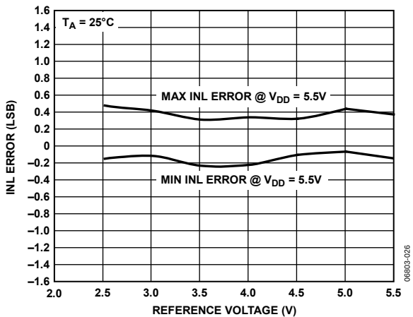
Figure 11. INL vs. Reference Input Voltage
