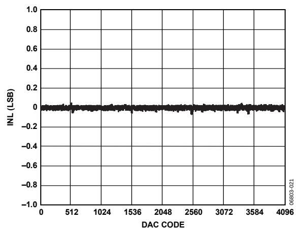
Figure 6. AD5024 INL
