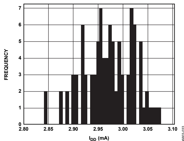
Figure 18. I_{DD} Histogram, V_{DD} = 5.0 V
