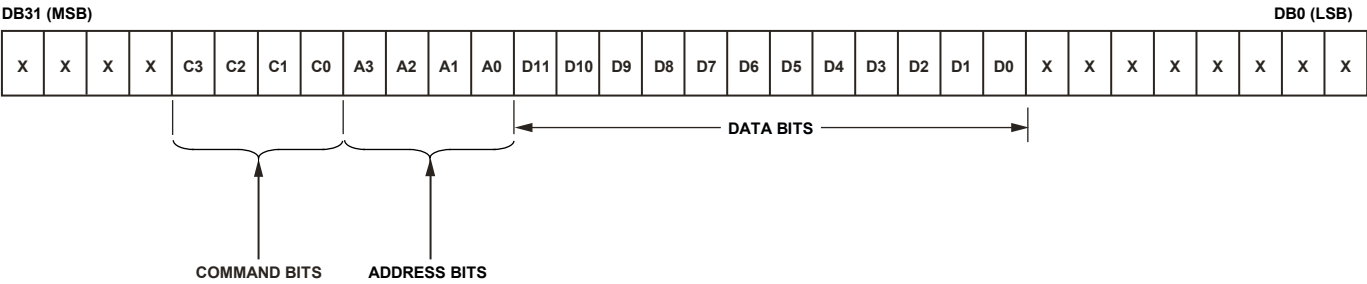
Figure 43. AD5024 Input Register Content
