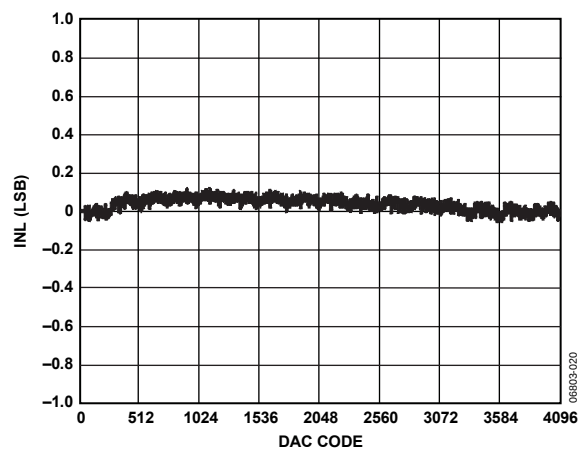
Figure 5. AD5044 INL
