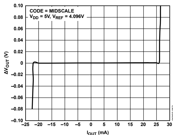
Figure 37. Typical Current Limiting Plot
