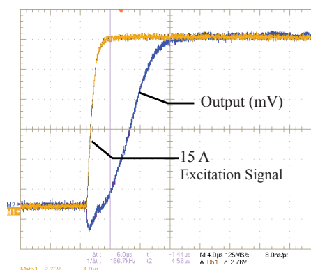
Step Response
