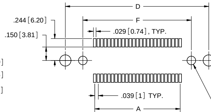
PCB LAYOUT CONNECTOR SIDE
