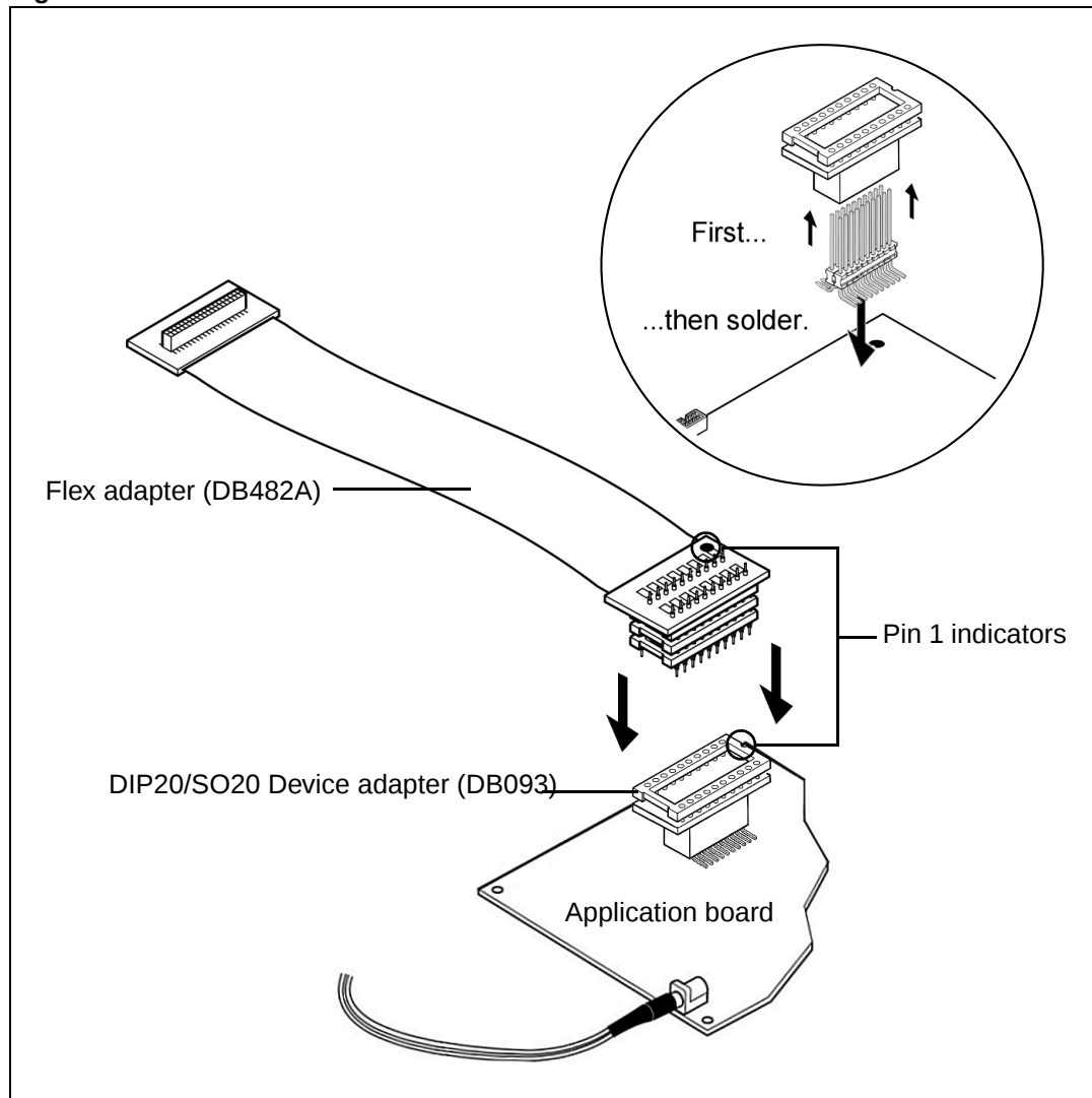
Figure 12. SO20 connection
