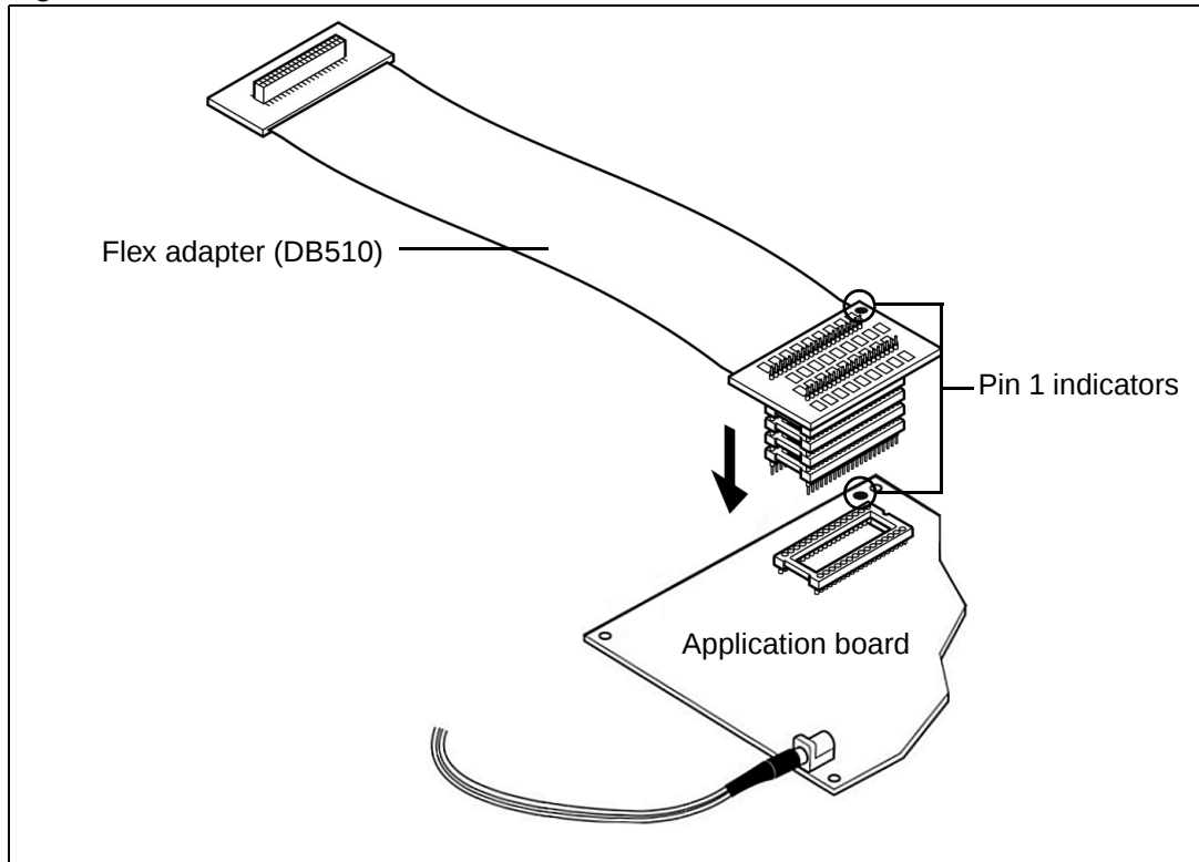
Figure 13. SDIP32 connection
