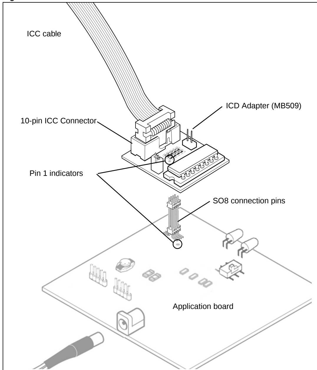
Figure 22. SO8 connection
