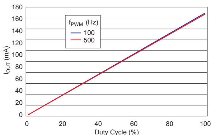
Figure 8. PWM pin dimming linearity.
