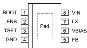
Pin-out Diagram
