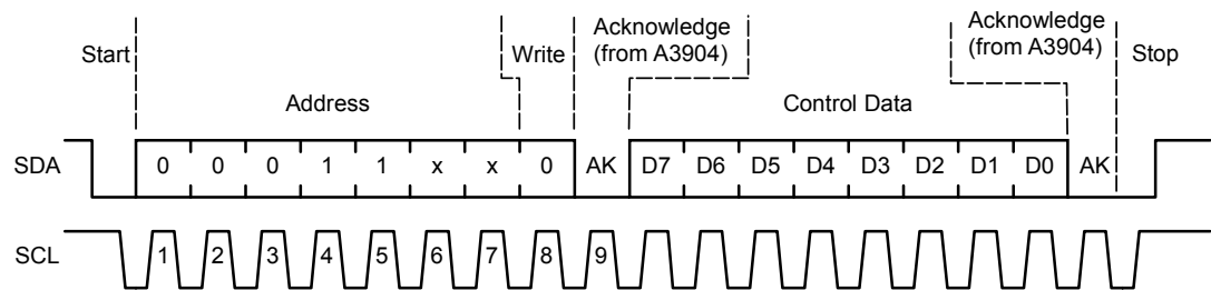
Write Register Bit Definition and Timing Diagram
