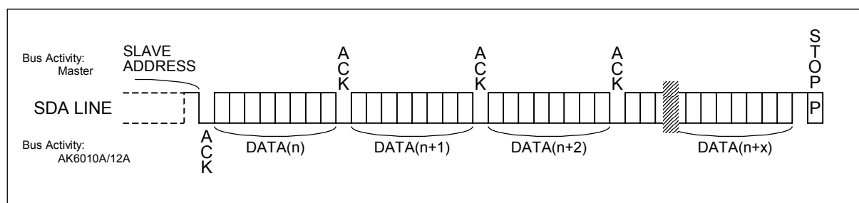
SEQUENTIAL READ
