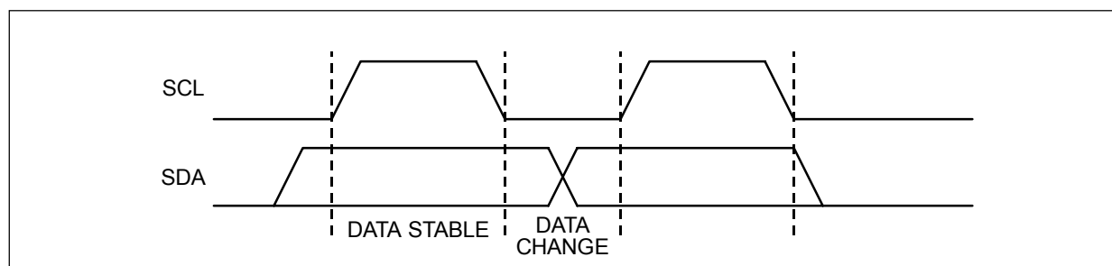
Figure 1. Data transfer
