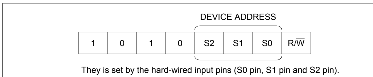
Figure 4. Slave Address
