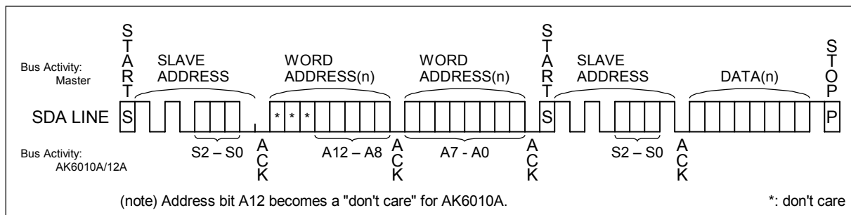
RANDOM READ
