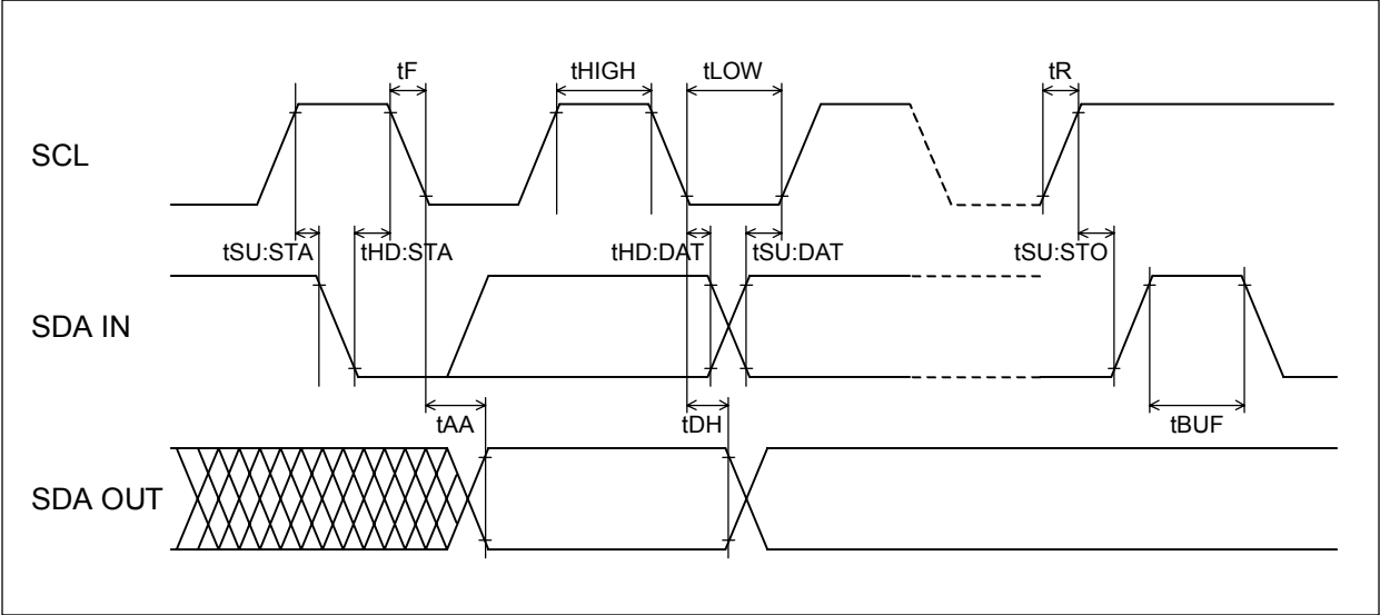
BUS TIMING
