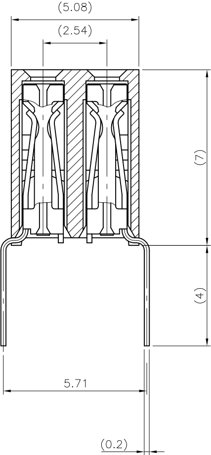
SECTION B-B
