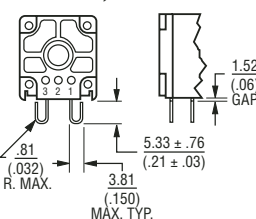
Model 94 J-Hooked Terminals, "L" Pattern
