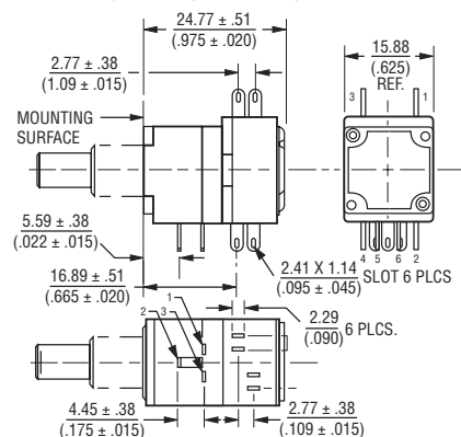
Model 99 1st Cup Same As Model 95 (2nd Cup - Switch)
