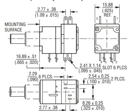
Model 97 1st Cup Same As Model 93 (2nd Cup - Switch)
