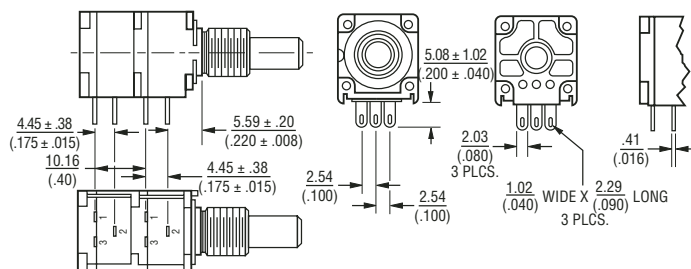
Model 95 Solder Lug Terminals, "Triangular" Pattern
