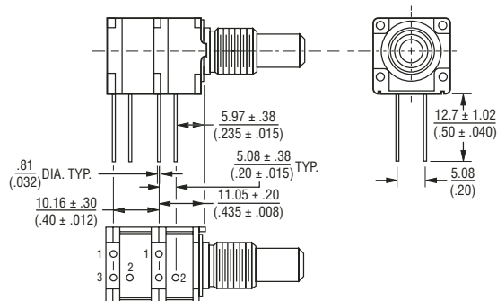
Model 93 PC Pin Terminals, "L" Pattern
