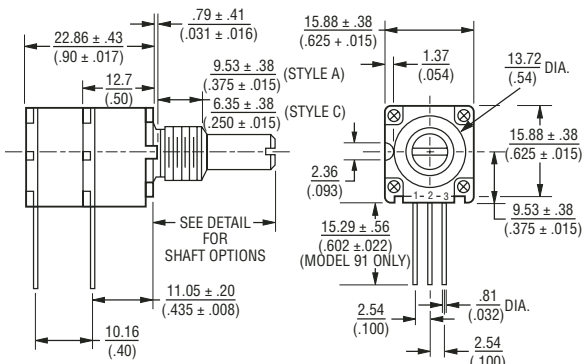
Model 91 & 96 PC Pin Terminals, In-Line
