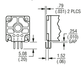
Model 94 J-Hooked Terminals, "L" Pattern
