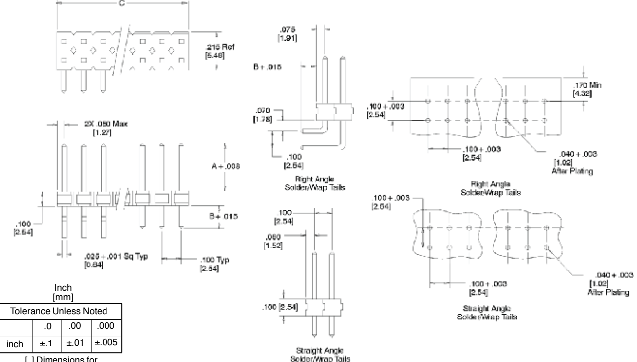
Recommended Hole Pattern
