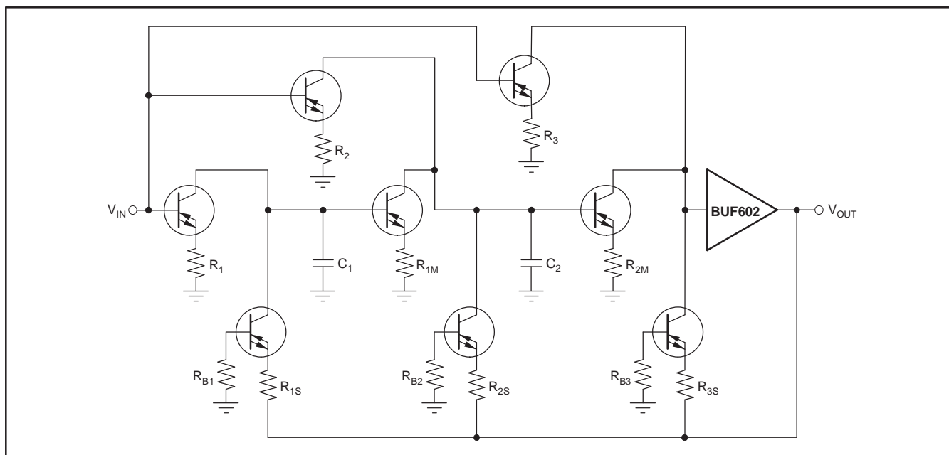
Figure 45. Universal Active Filter
