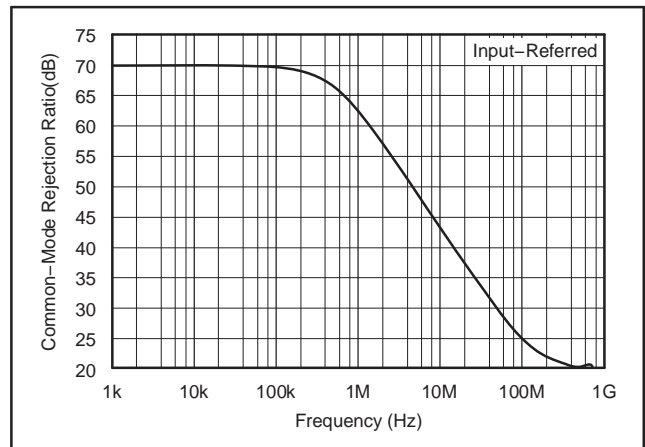
Figure 49. CMRR of the ADC Driver
