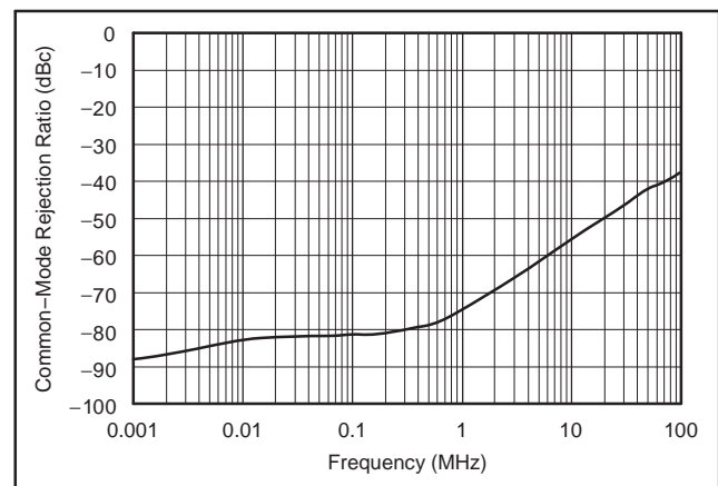
Figure 40. Differential Driver Common-Mode Rejection Ratio for 2V PP Input Signals
