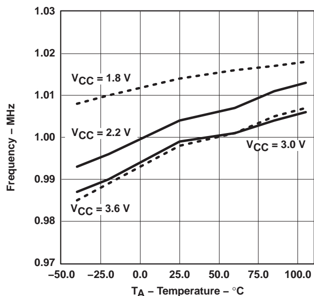
Figure 11. Calibrated 1 MHz Frequency vs. Temperature
