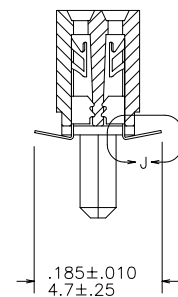
SECTION X-X
