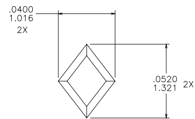
VIEW E-E SCALE 40/1
