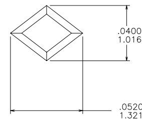
VIEW F-F SCALE 40/1
