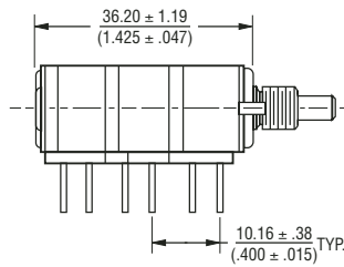
Triple Unit - PC Pins & J-Hook
