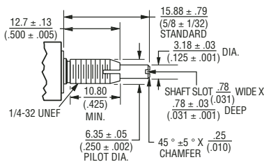
"E" Bushing 1/4 " (6.35 mm) Dia. Locking - Single Shaft
