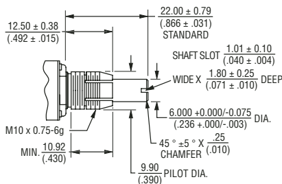
"S" Bushing 10 mm Dia. Locking - Single Shaft
