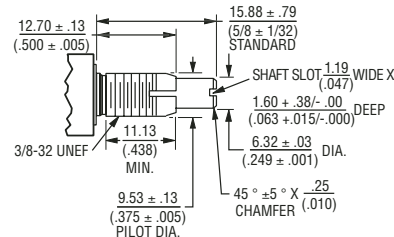
"B" Bushing 3/8 " (9.53 mm) Dia. Plain - Single Shaft
