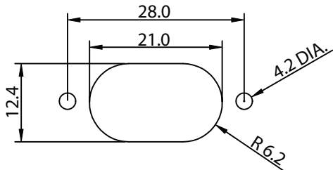
PANEL CUTOUT
