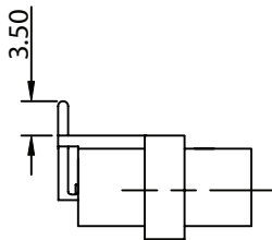
PCB MOUNTING
