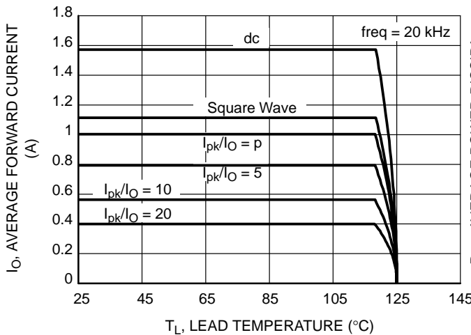
Figure 5. Current Derating
