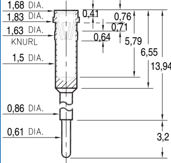
1306-0-15-XX-47-XX-04-0 Press-fit in 1,55 mounting hole.
