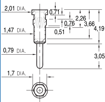
8401-0-15-XX-47-XX-04-0 Hex press-fit in 1,6 plated thru hole
