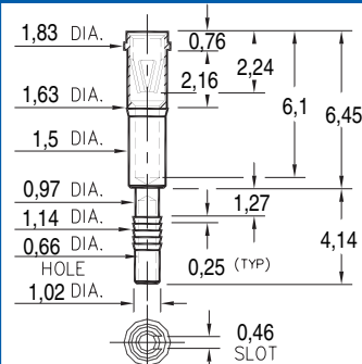
4615-0-31-XX-47-XX-04-0 Compliant press-fit in 1,02±0,08 plated hole. For 2,29" 3,30 thick board.
