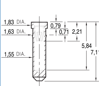
6857-0-15-XX-47-XX-10-0 Press-fit in 1,55 mounting hole.
