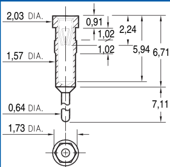
0335-0-15-XX-47-XX-04-0 Hex press-fit in 1,63 plated thru hole
