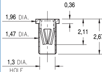
7305-0-15-XX-47-XX-10-0 Solder mount in 1,52 min. mounting hole Also available on 24mm wide carrier tape: 1,500 parts per 330mm reel. Order as: 7305-0-57-XX-47-XX-10-0
