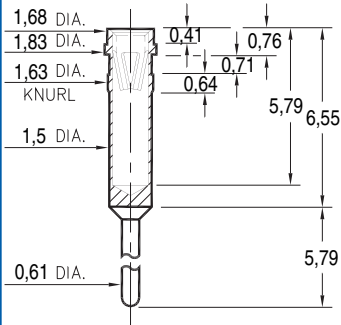
1305-0-15-XX-47-XX-04-0 Press-fit in 1,55 mounting hole
