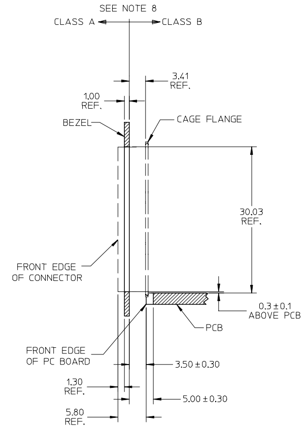
SECTION Z-Z
