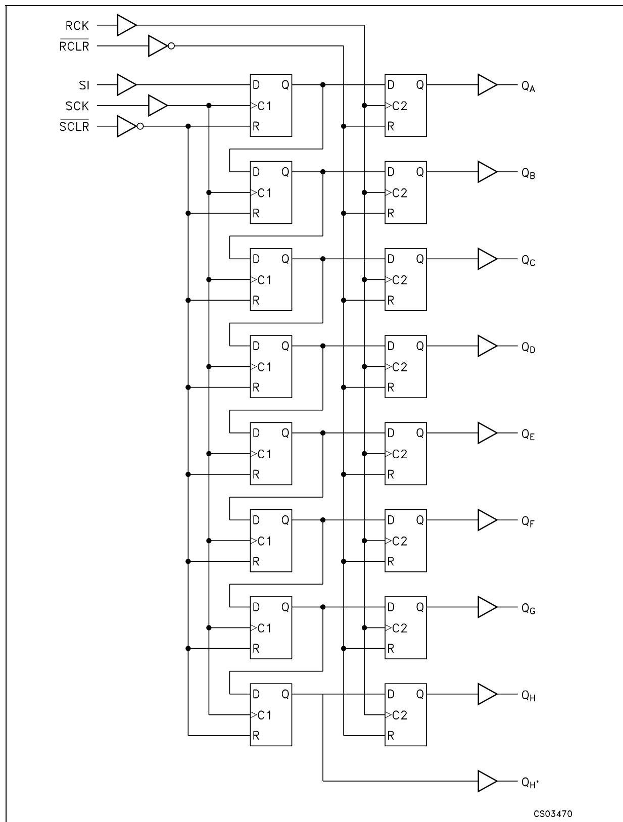
Figure 3: Logic Diagram
