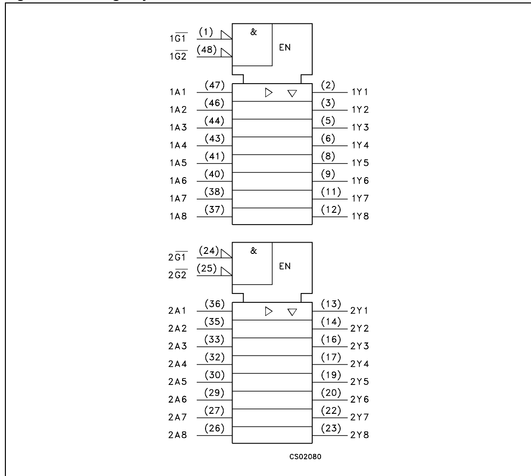
Figure 1. IEC logic symbols
