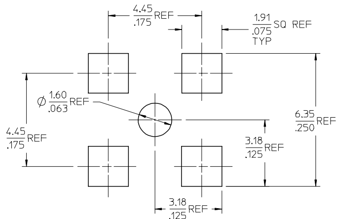
RECOMMENDED MOUNTING PATTERN
