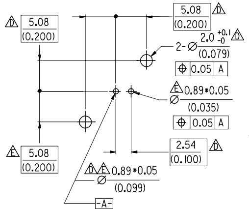
PCB HOLE CONFIGURATION
