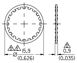
LOCK WASHER
