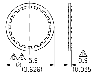
LOCK WASHER
