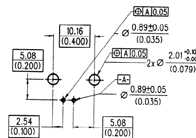
PCB HOLE CONFIGURATION
