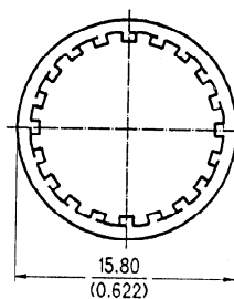
LOCK WASHER
