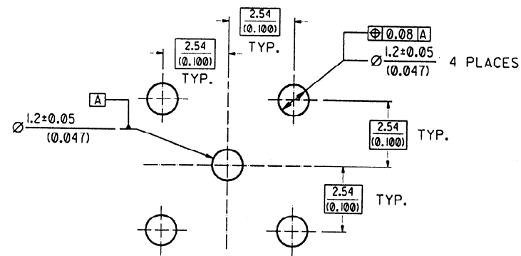
RECOMMENDED PCB MOUNTING HOLE
