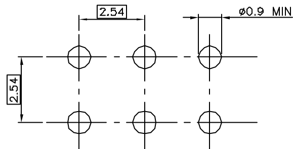
RECOMMENDED HOLE PATTERN
