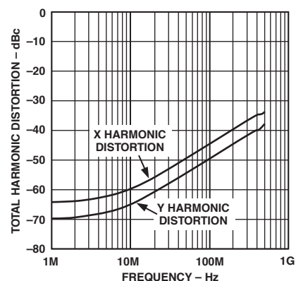
TPC 3. Total Harmonic Distortion vs. Frequency
