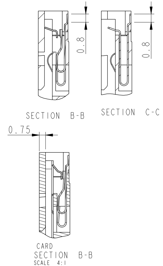
DETAIL OF SWITCH
